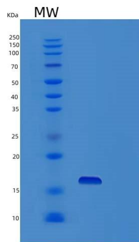
Figure . SDS-PAGE
