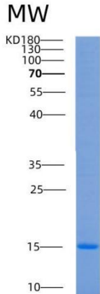
Figure 1. SDS-PAGE
