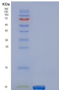
Figure 1. SDS-PAGE
