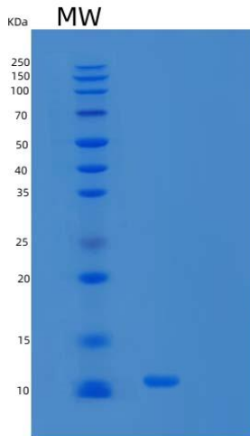
Figure 1. SDS-PAGE
