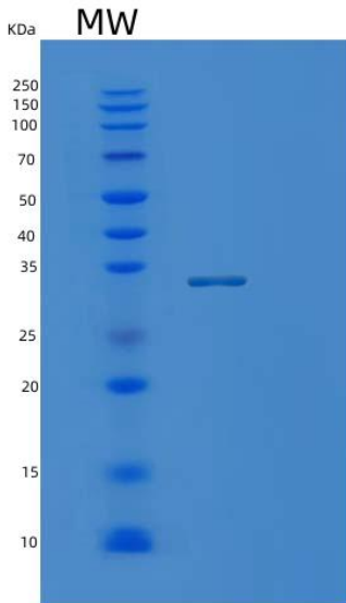
Figure 1. SDS-PAGE
