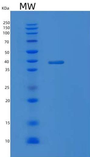
Figure 1. SDS-PAGE
