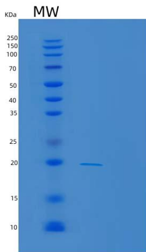
Figure 1. SDS-PAGE
