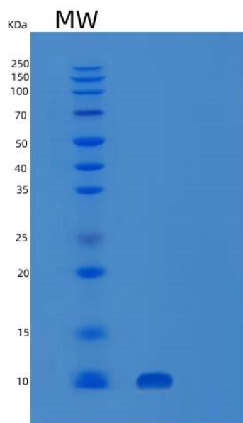
Figure . SDS-PAGE
