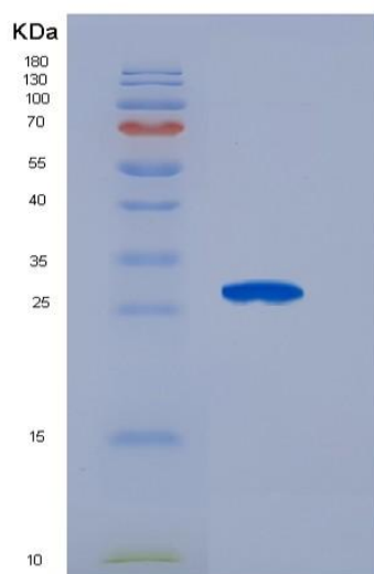
Figure . SDS-PAGE
