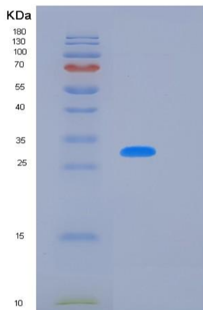
Figure . SDS-PAGE
