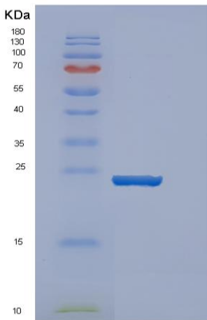
Figure 1. SDS-PAGE
