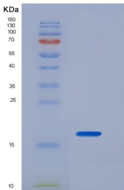
Figure . SDS-PAGE
