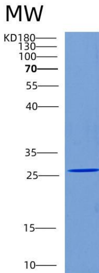
Figure 1. SDS-PAGE
