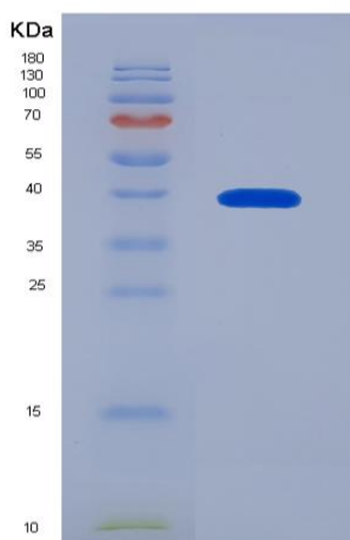
Figure 1. SDS-PAGE
