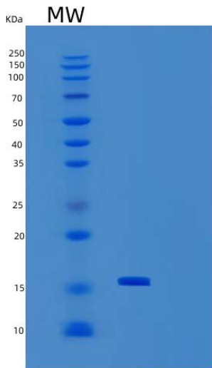
Figure 1. SDS-PAGE
