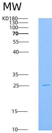
Figure 1. SDS-PAGE
