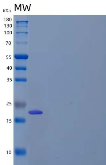
Figure 1. SDS-PAGE
