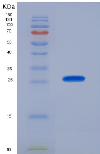
Figure 1. SDS-PAGE
