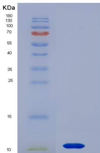
Figure 2. SDS-PAGE
