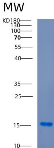
Figure 1. SDS-PAGE
