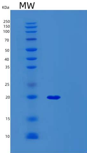
Figure 1. SDS-PAGE
