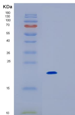
Figure 2. SDS-PAGE
