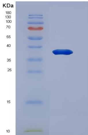
Figure 1. SDS-PAGE
