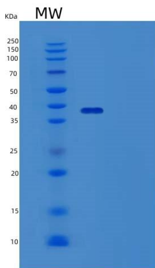
Figure . SDS-PAGE
