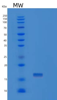
Figure 1. SDS-PAGE
