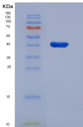
Figure 2. SDS-PAGE
