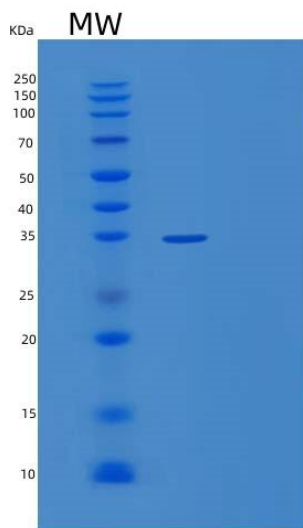
Figure 1. SDS-PAGE
