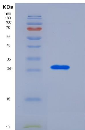
Figure . SDS-PAGE
