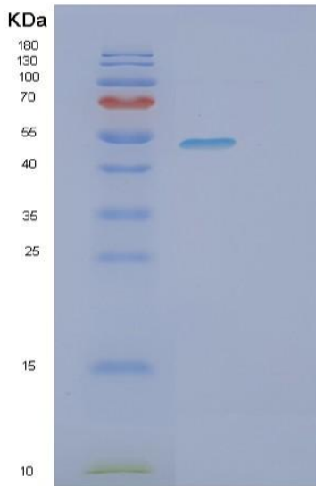
Figure 2. SDS-PAGE
