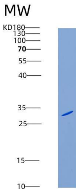
Figure 1. SDS-PAGE
