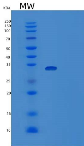
Figure 2. SDS-PAGE
