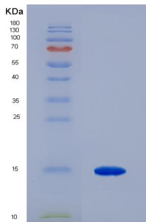
Figure 1. SDS-PAGE
