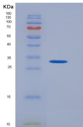
Figure 1. SDS-PAGE
