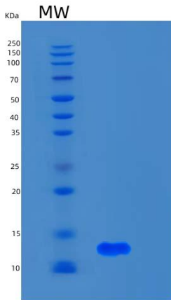
Figure 1. SDS-PAGE
