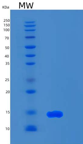
Figure 1. SDS-PAGE
