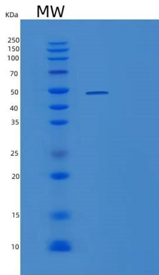
Figure . SDS-PAGE
