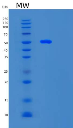
Figure 1. SDS-PAGE
