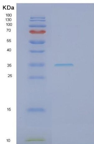
Figure 1. SDS-PAGE
