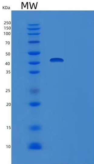
Figure 1. SDS-PAGE
