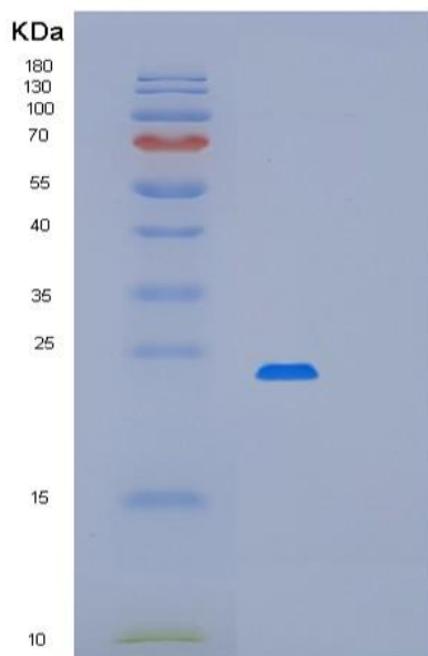
Figure . SDS-PAGE
