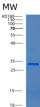
Figure 1. SDS-PAGE
