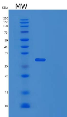
Figure 1. SDS-PAGE
