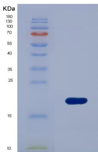
Figure . SDS-PAGE
