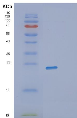
Figure . SDS-PAGE
