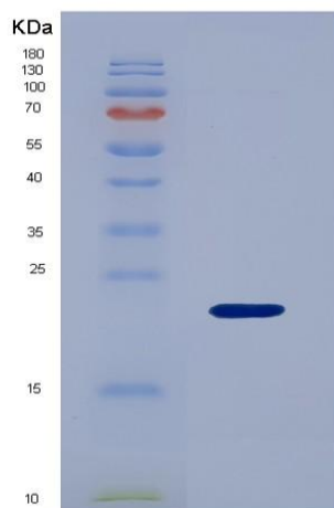
Figure . SDS-PAGE
