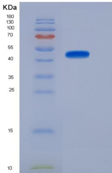
Figure . SDS-PAGE
