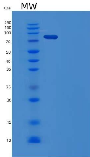
Figure . SDS-PAGE
