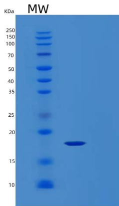
Figure 1. SDS-PAGE
