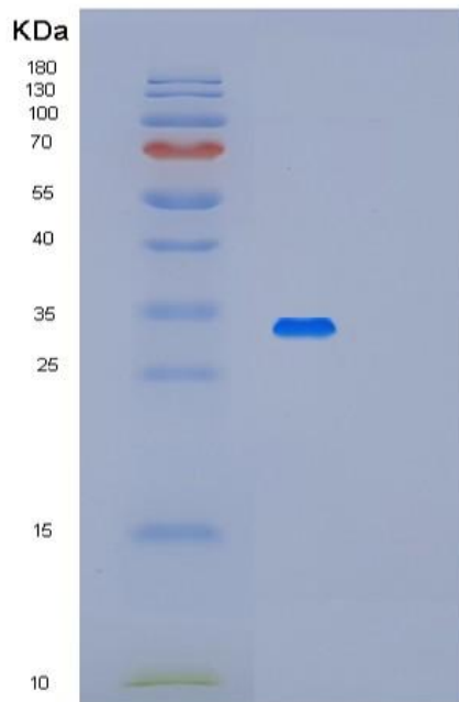
Figure . SDS-PAGE
