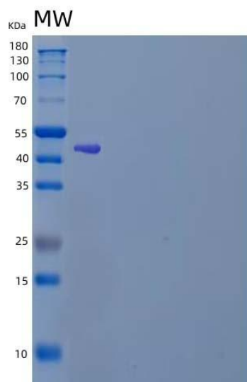
Figure 1. SDS-PAGE
